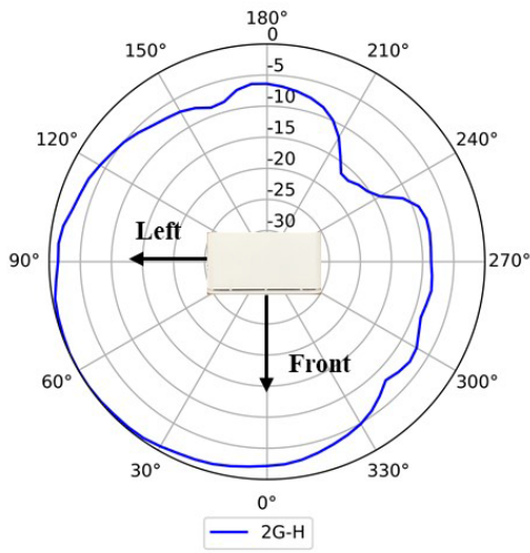
2.4GHz (Horizontal)
